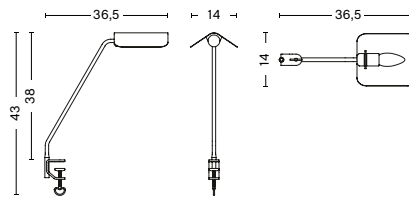
APEX DESK CLIP LAMP WIDTH 14 CM DEPTH 36,5 CM HEIGHT 43 CM MAX. TABLE/SHELF THICKNESS 4 CM
