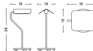
APEX TABLE LAMP WIDTH 19 CM DEPTH 16 CM HEIGHT 38 CM
